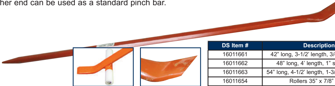
with rollers
