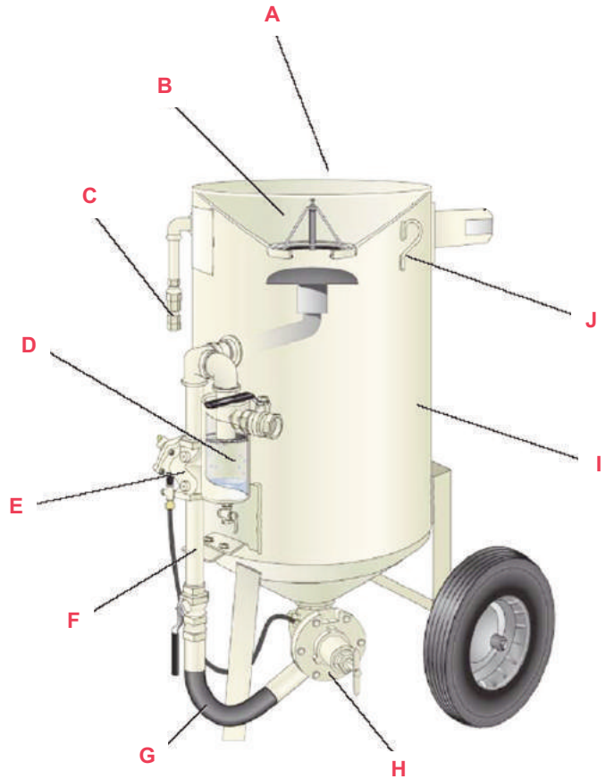
Portable unit shown. No wheels on stationary unit.
